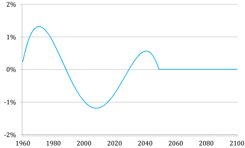
Figure 1: Fertility rates used in the model
