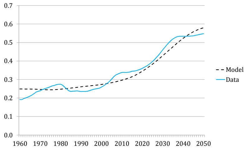
Figure 2: Old age dependency ratio (>65 / 20-64) in Germany
