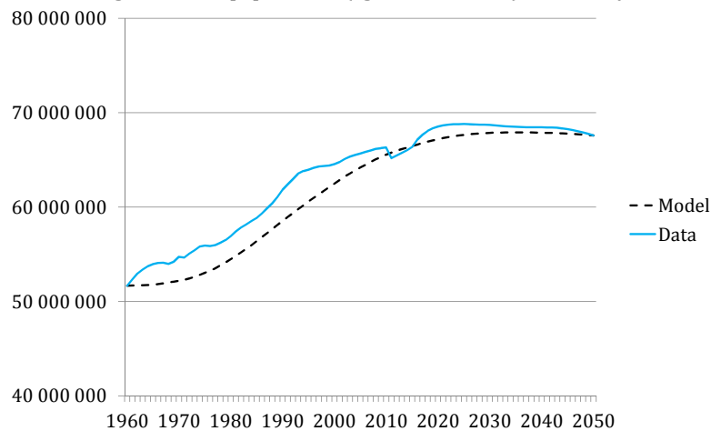
Figure 3: Total population (aged 20 and more) in Germany
