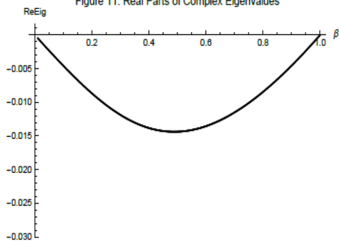
Figure 11: Real Parts of Complex Eigenvalues
